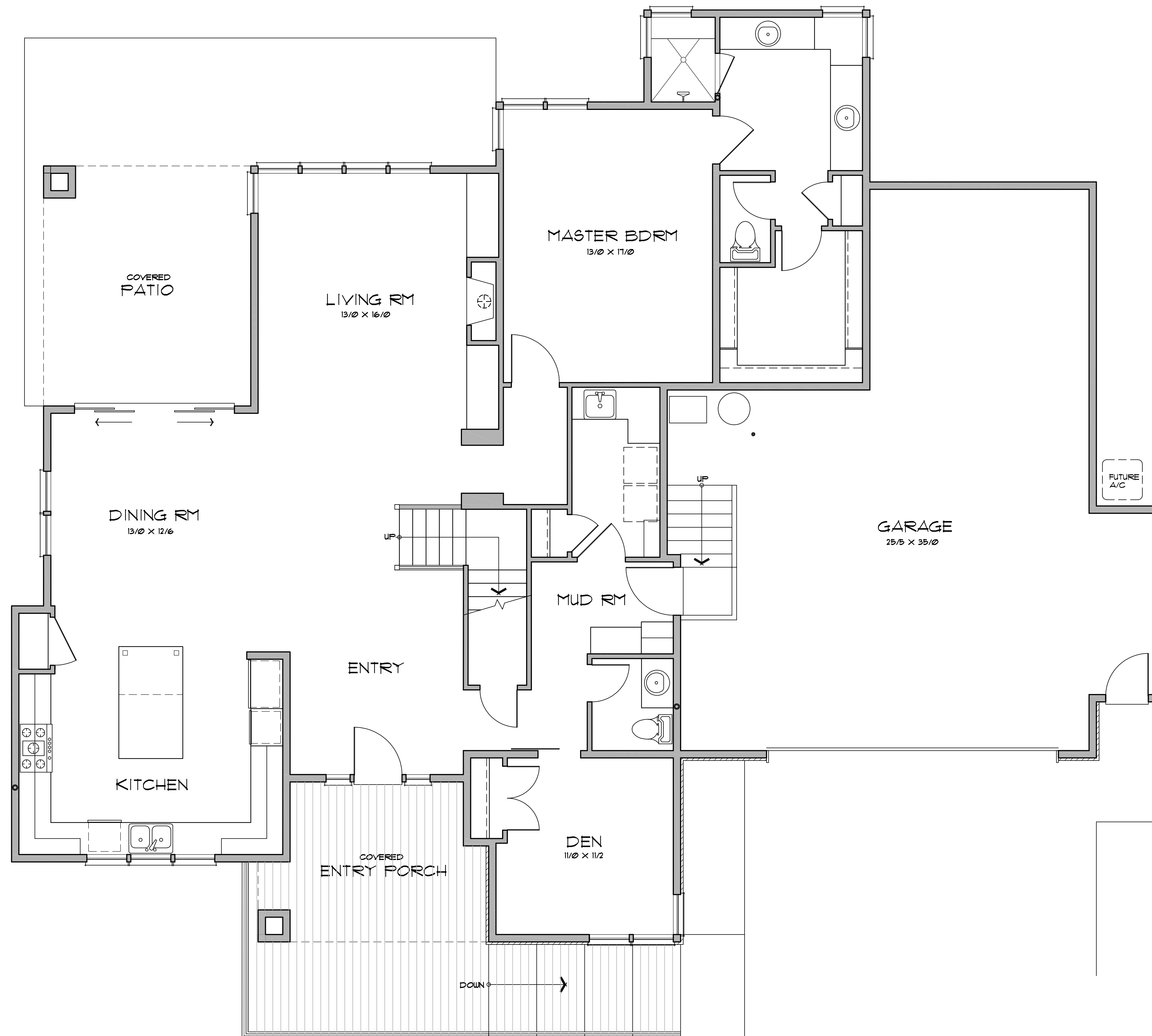
MAIN LEVEL FLOOR PLAN
